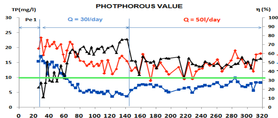
Figure 8. TP treatment efficiency
