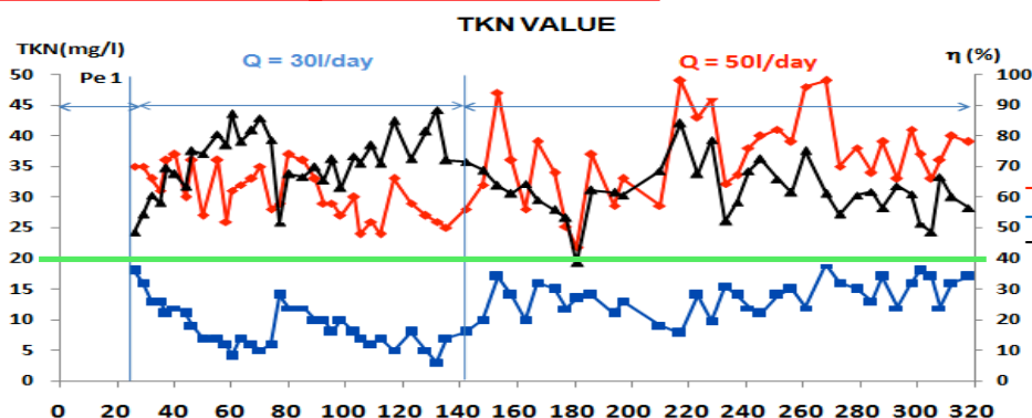
Figure 7. TKN treatment efficiency
