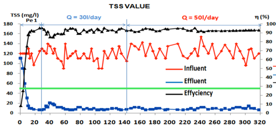
Figure 4. TSS treatment efficiency
