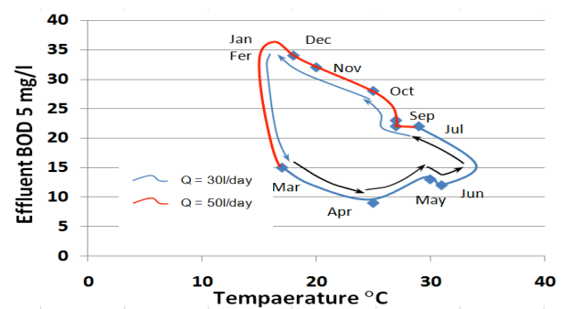
Figure 3. Relationship between BOD and temperature
