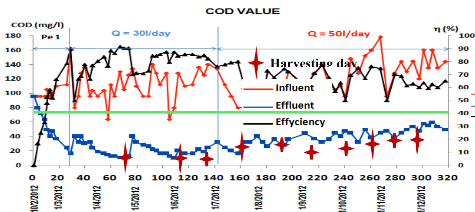
Figure 5. COD treatment efficiency
