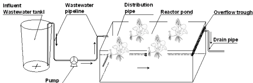
Figure 2. Reactor system (aquatic pond made by safety glass)
